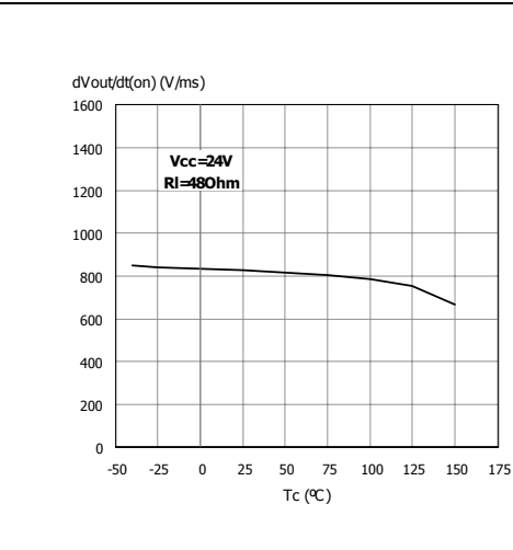
Figure 13. Turn-on voltage slope
