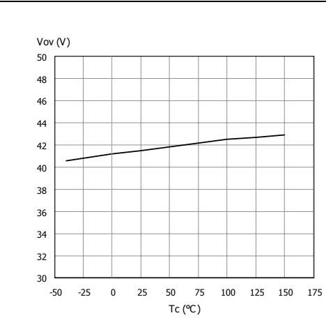
Figure 13. Turn-on voltage slope
